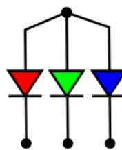
LED RGB Anode Commune
